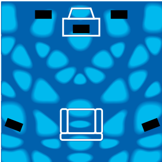
Conventional home cinema systems
